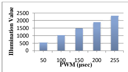
Fig.8. PWM versus Illumination
