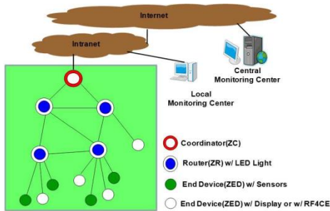
Fig. 2. ZigBee Network
