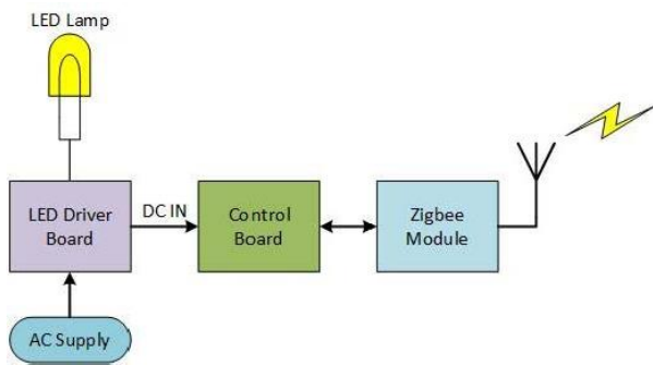
Fig.5. Transmitter Block Diagram
