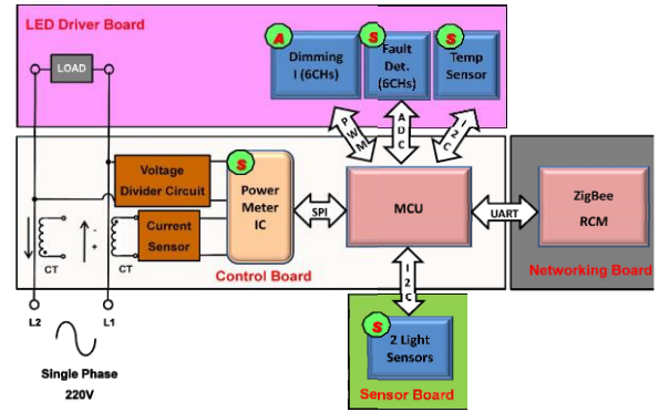
Fig.3. Node Block Diagram
