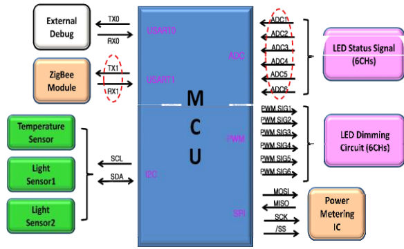
Fig.4. MCU Communication Block Diagram
